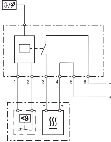
Connection diagram
